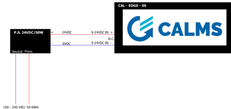
Photo 1: Electrical schematic of the CAL-EDGE-0 device
