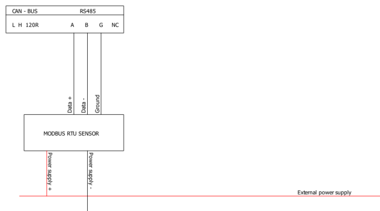
Photo 2: Connection of MODBUS sensors to the CAL-EDGE-0 device
